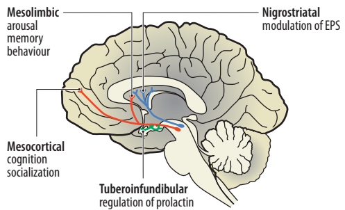
Fig. 12.3.3: Antipsychotics work on the mesolimbic and mesocortical dopamine pathways to inhibit positive and negative symptoms of schizophrenia, respectively. Antipsychotics cause EPSE via the nigrostriatal pathway and endocrine side effects via the tuberoinfundibular pathway .
