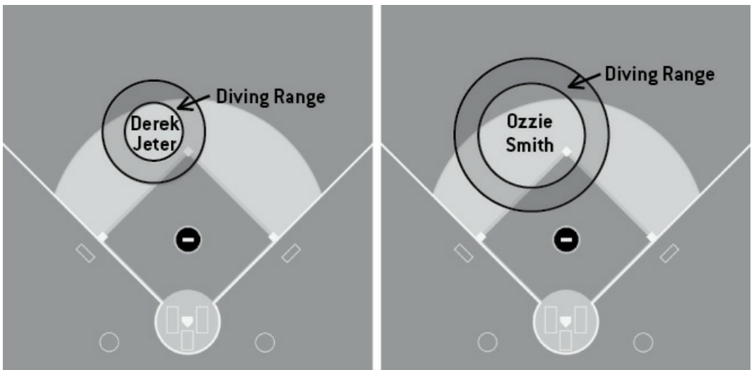
FIGURE C-1: SHORTSTOP DIVING RANGES
