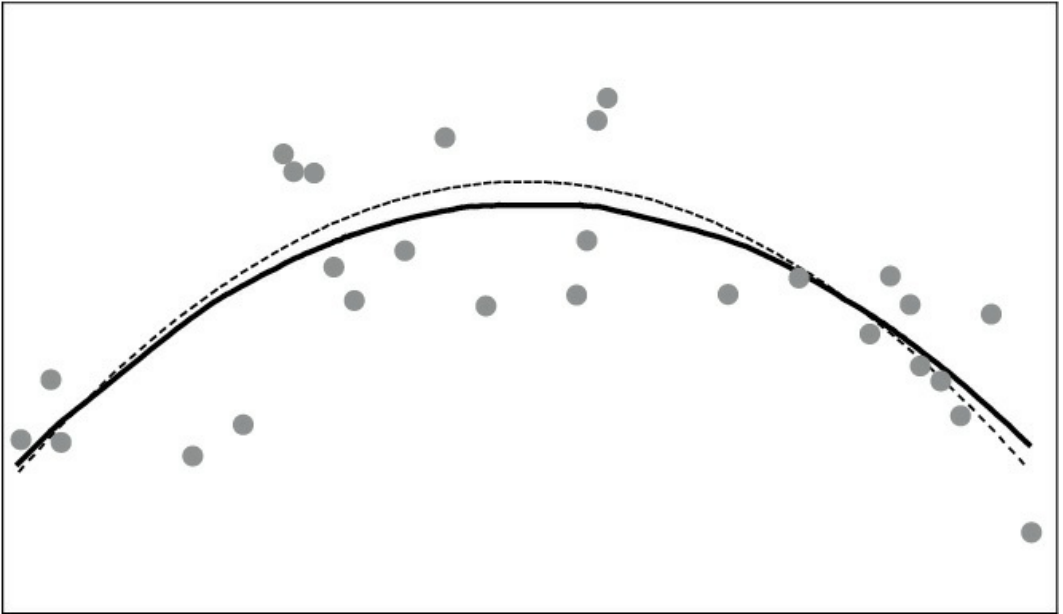
FIGURE 5-6B: WELL-FIT MODEL
