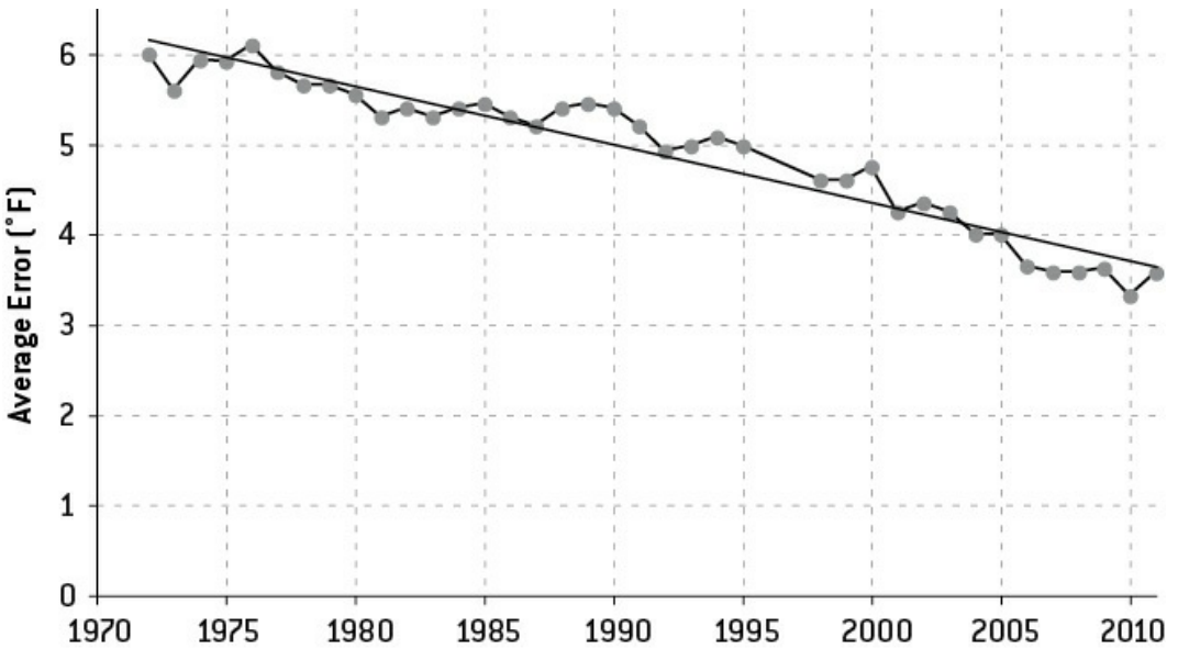
FIGURE 4-4: AVERAGE HIGH TEMPERATURE ERROR IN NWS FORECASTS
