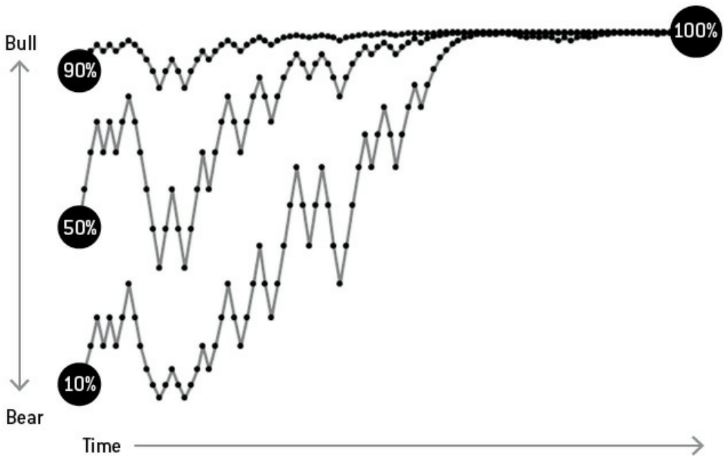
FIGURE 8-8: BAYESIAN CONVERGENCE
