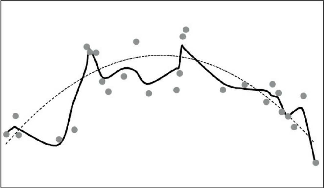
FIGURE 5-6C: OVERFIT MODEL
