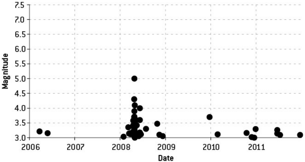
FIGURE 5-4D: EARTHQUAKES NEAR RENO, NEVADA JANUARY 1, 2006–DECEMBER 31, 2011
